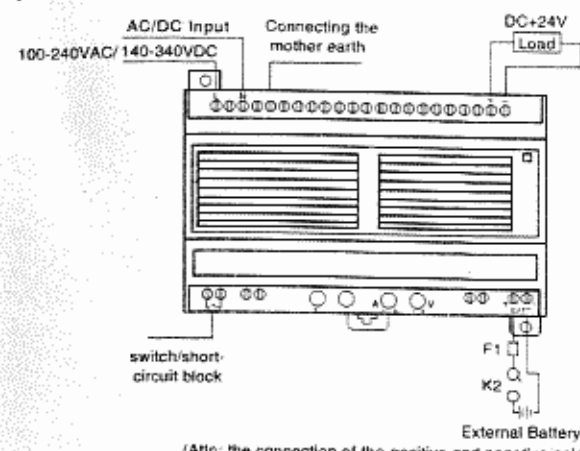
(Fig 3.3 UPS application)
